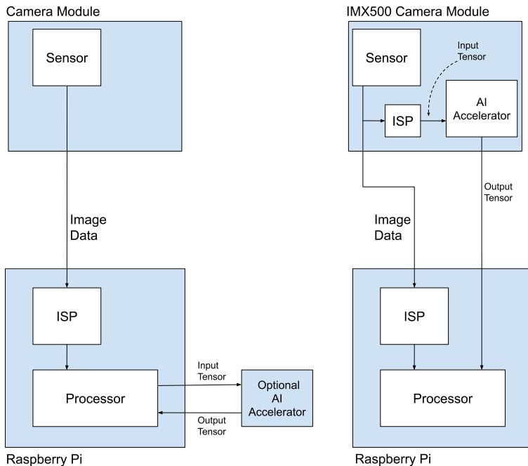
◀ Figure 3: Camera Module vs AI Camera Module ▼ Figure 4: The various software components (green) and Raspberry Pi hardware components (red)
