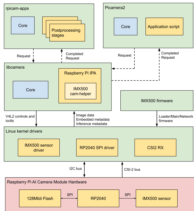
◀ Figure 3: Camera Module vs AI Camera Module ▼ Figure 4: The various software components (green) and Raspberry Pi hardware components (red)
