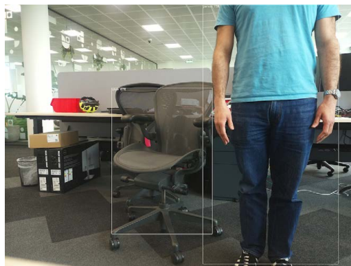
Figure 1: Object detection
